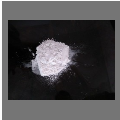
Carboxymethyl Cellulose
